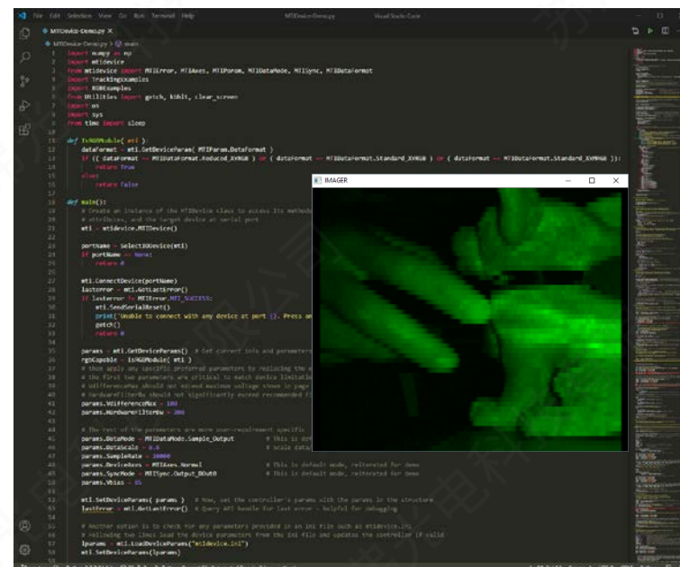
Python SDK in Windows example: Development Kit with Tracking Bundle Add-On used in Laser Imaging Mode
