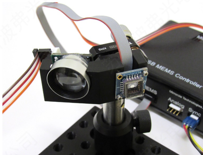
Laser Tracking Bundle Add-On in use with a Standard Devkit's 2mm MEMS Mirror A7M20.2-2000AL-TINY20.4. Mirror is co-mounted with a Tracking Photosensor addressing a common Field of View.
